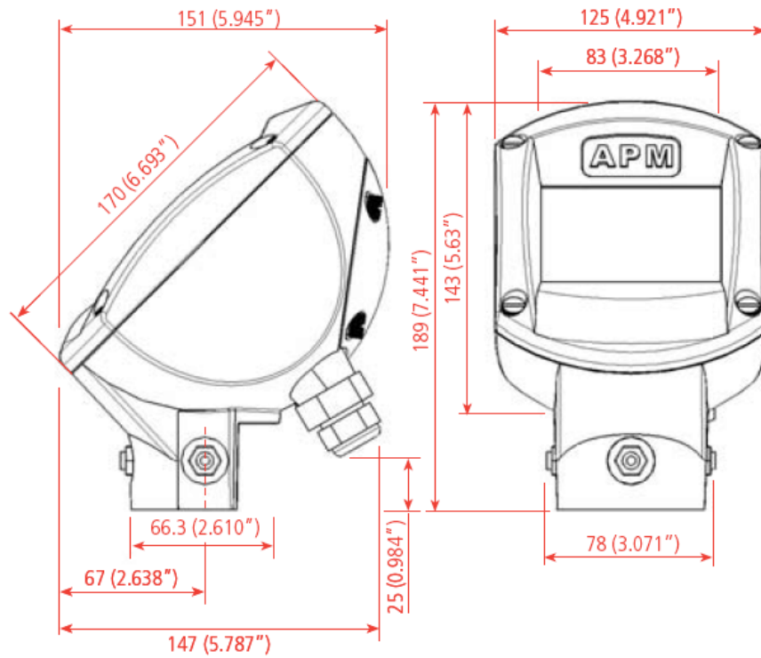
Figure 11: 3DLevelScanner S housing
