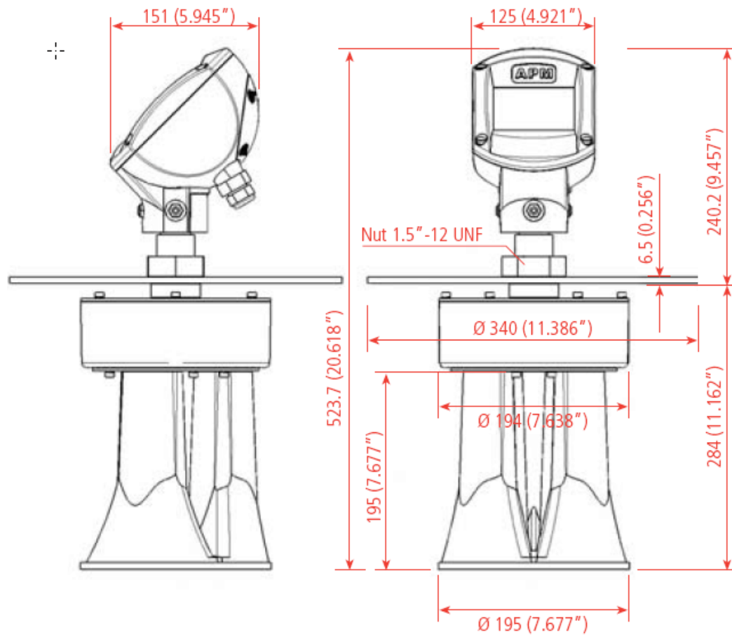
Figure 10: 3DLevelScanner S with horn antenna in flange version
